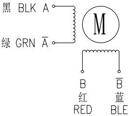
电机接线Motor Wiring Diagram
